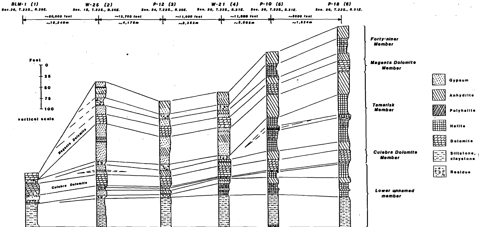
Figure 2.--Columnar cross section across WIPP site showing lithologic correlations of units in Rustler Formation.
