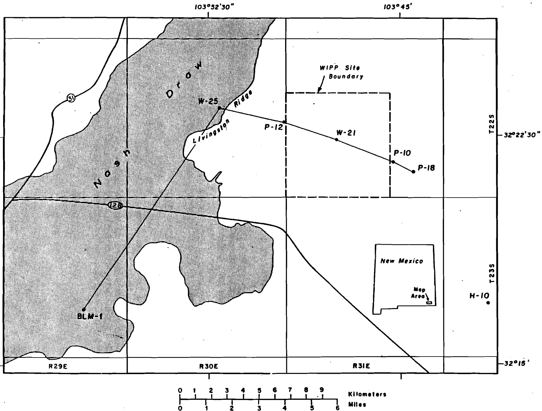
Figure 1.-- Location of Waste Isolation Pilot Plant (WIPP) site, southeastern New Mexico, and line of section shown on figure 2.
